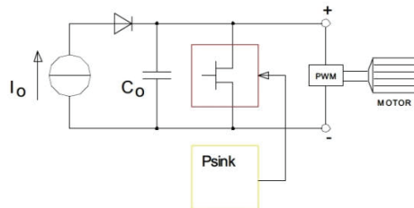
PSINK equipped power supply: absorbs breaking energy
