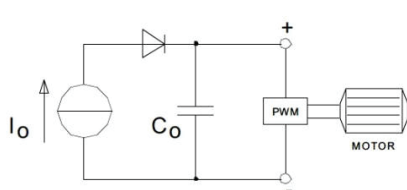
Conventional power supply: breaking power charges output capacitor C_o
