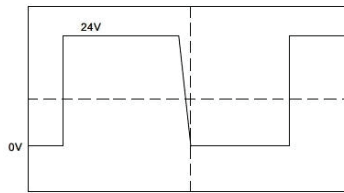
Latency of PSINK equipped power supply
