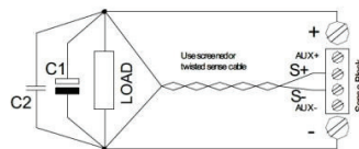
Remote Sensing (fig.6)
