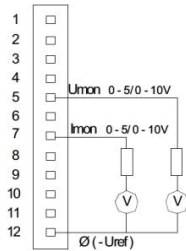
Monitor Output Connections (fig.2)
