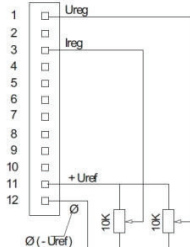
Program Input Connections (fig.4) (example with external poti)
