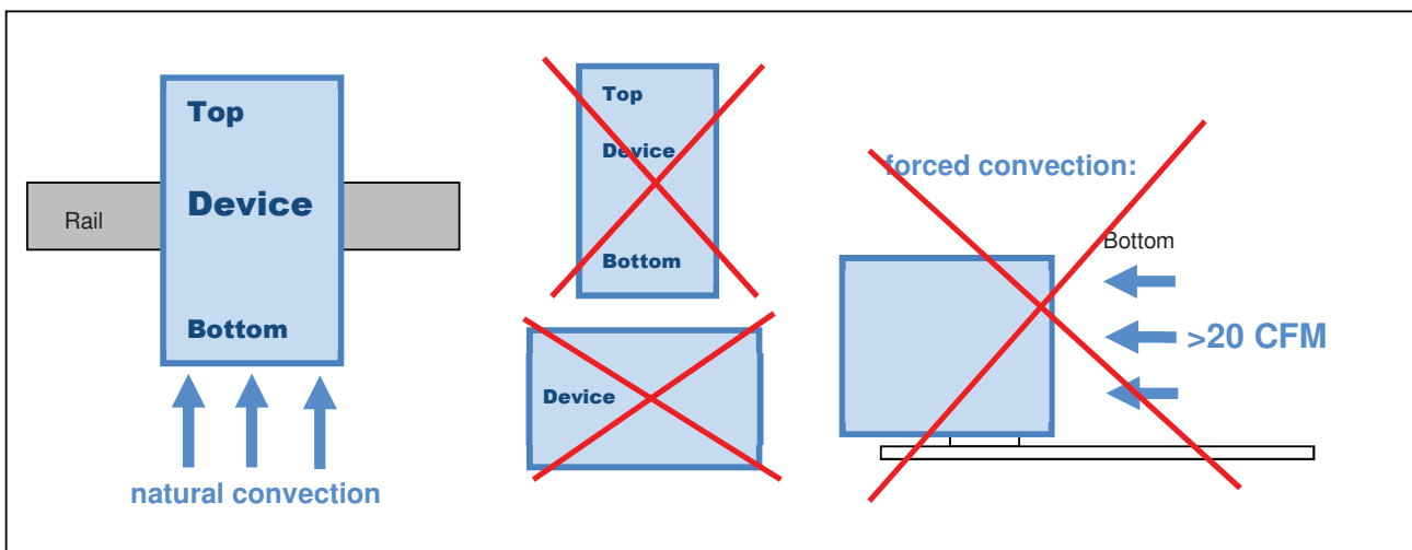
Mounting Instruction
